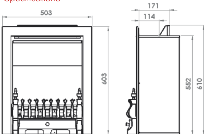
Paragon P3 Hybrid Elite Trim & Gate Fret in Chrome
